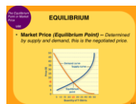
PPT 2-27 Equilibrium
