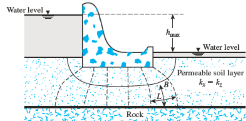
Figure 2.12 Flow net
