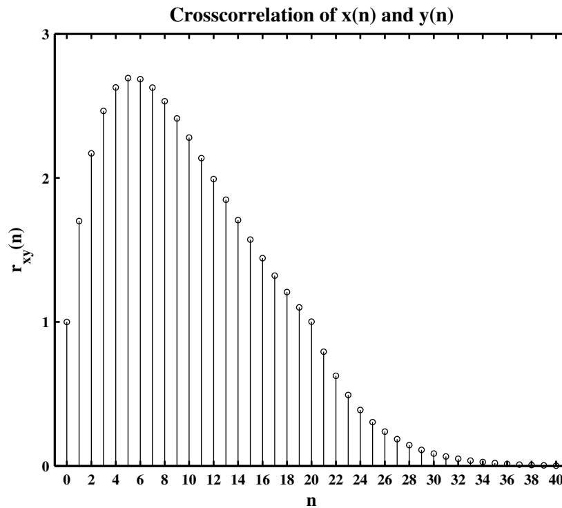
Figure 2.31: Problem P2.9 crosscorrelation plot
