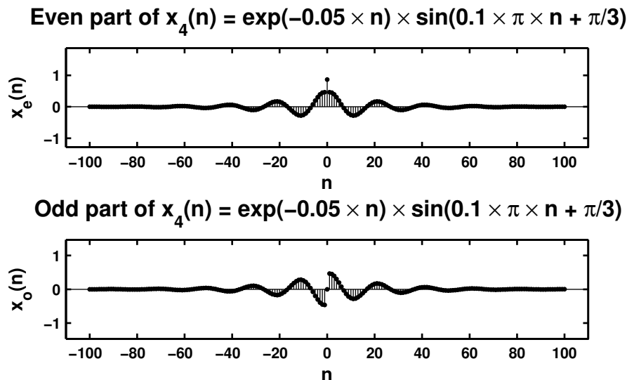
Figure 2.26: Problem P2.6.1 sequence plot
